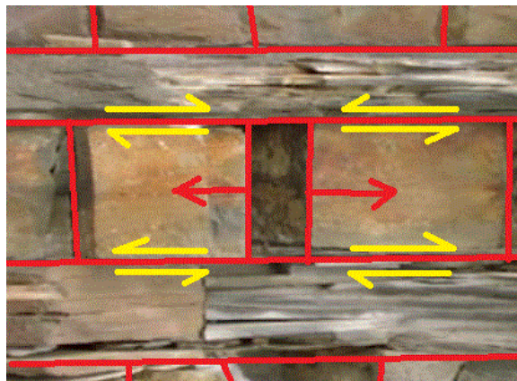
Figure 4: This is a conceptual model of shear failure (yellow arrows) along weak planes (red lines) in shales driven by hydraulic opening of vertical cracks (red arrows).
