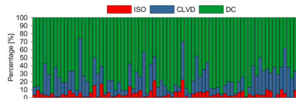
Figure 2: Products of decomposition for inverted 75 full moment source mechanisms.
