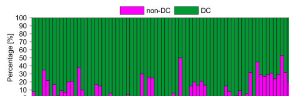
Figure 5: Minimal real percentages of non-shear components (magenta) for inverted 75 full moment source mechanisms.
