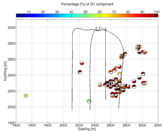
Figure 3: Map view of 75 source mechanisms colored according to their real percentage of DC component.
