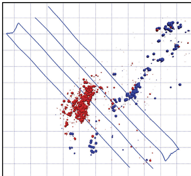
Figure 7 Map of microseismicity generated during a 24-hour period. Events are sized by moment magnitude and coloured by source mechanism. Red events are dip-slip associated with fracture stimulation and blue events are strike-slip related with fault activation. Grid squares are 500' x 500 ft.
