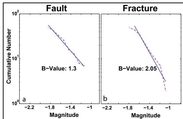
Figure 6 Cumulative FMD plots for individual cells indicated in Figure 4. (a) The lower b value of 1.3 indicates that the cell is dominated by fault activity. (b) The fracture cell b value of 2.05 indicates greater fracture stimulation.
