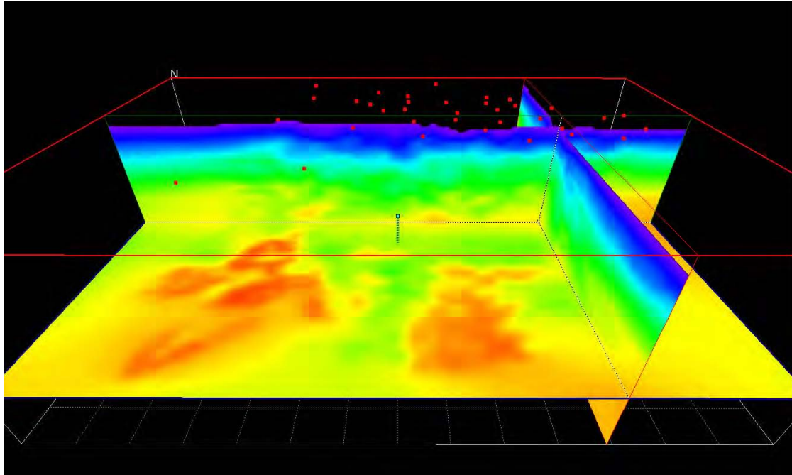
Figure 3: Result of velocity inversion of arrival time data for events in Figure 2. Hotter colors are faster velocities. Horizontal slice is at 2 km depth. Red dots are the station locations. Two basins structures are seen separated by a valley.
